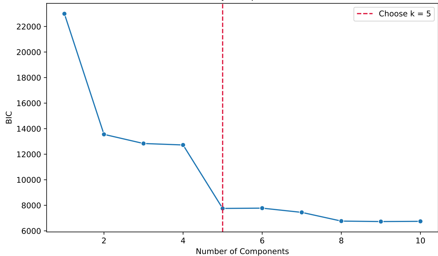
GMM BIC by Component Count
